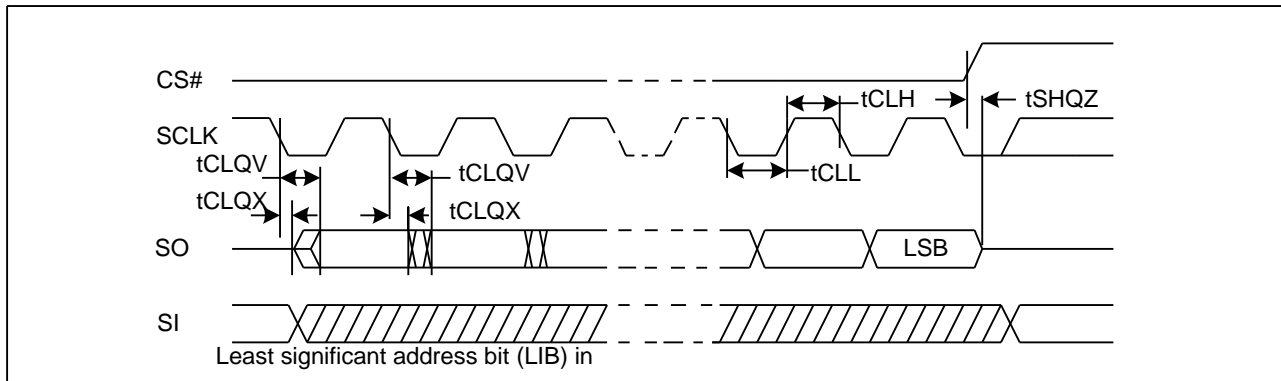
Figure36. Output Timing
