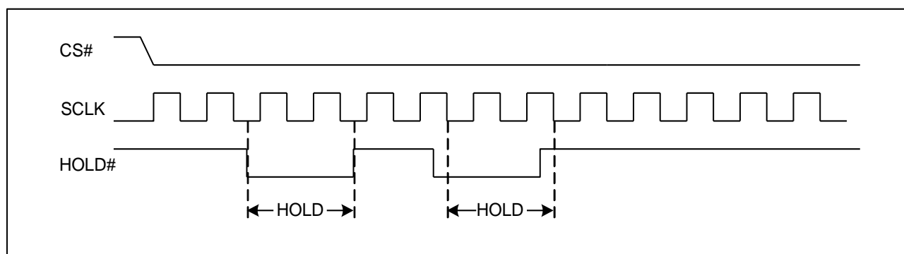
Figure1. Hold Condition
