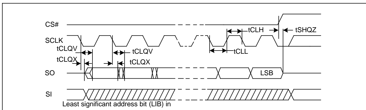
Figure 41. Output Timing
