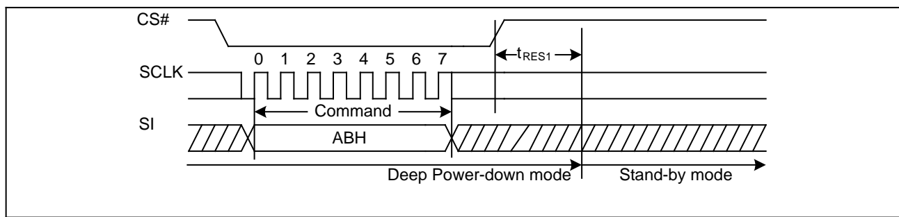
Figure 27. Release Power-Down/Read Device ID Sequence Diagram
