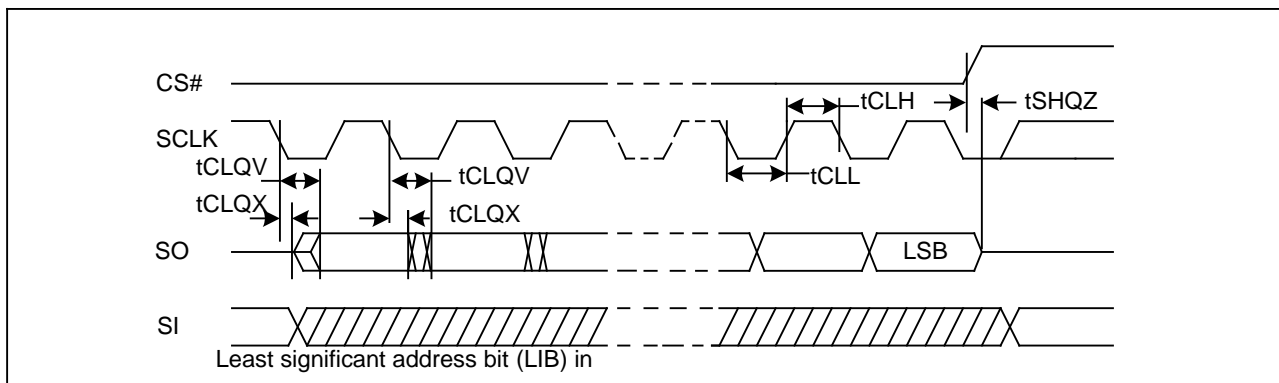
Figure36. Output Timing
