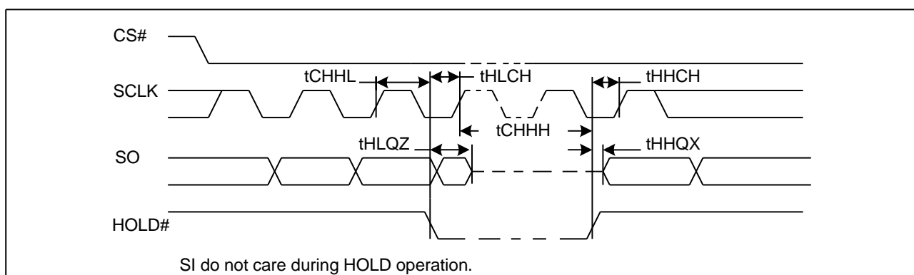
Figure51. Hold Timing
