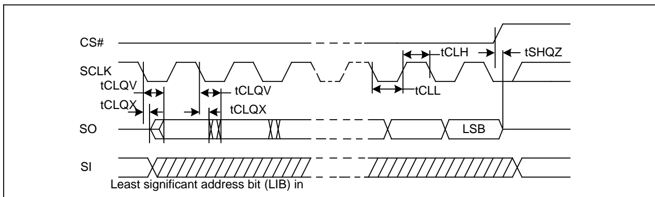
Figure 30. Output Timing
