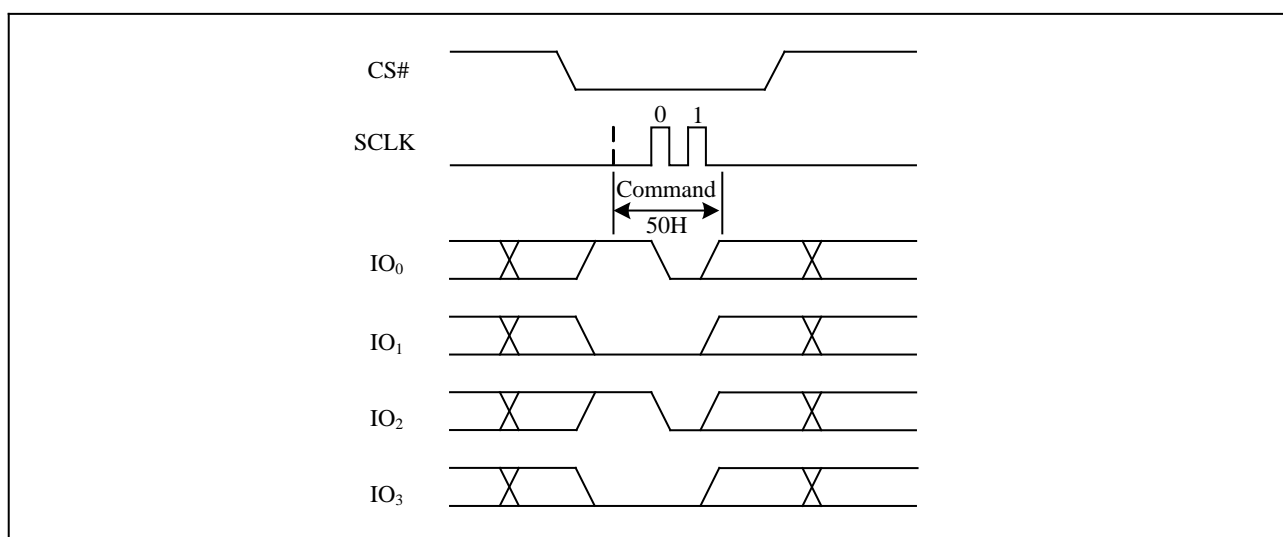
Figure4a. Write Enable for Volatile Status Register Sequence Diagram (QPI)
